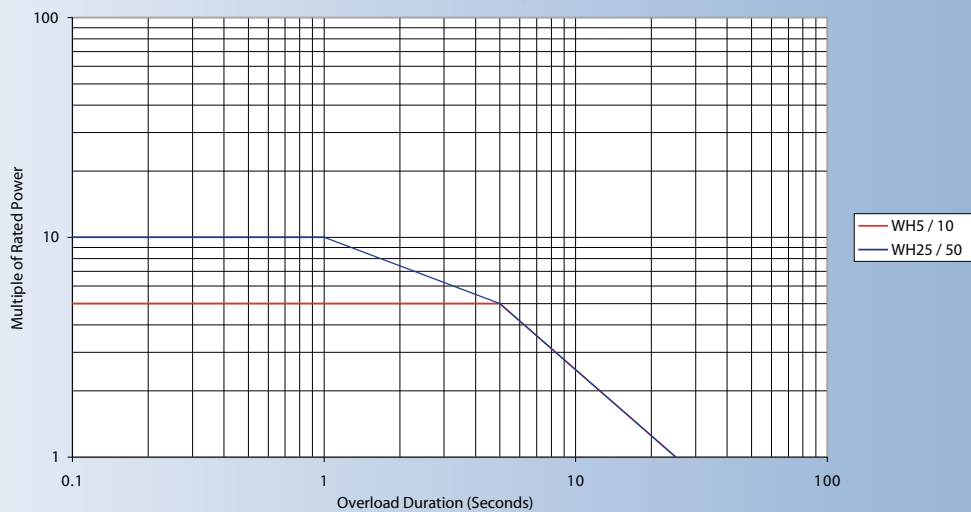
WH Series "Overload Rating" Graph
