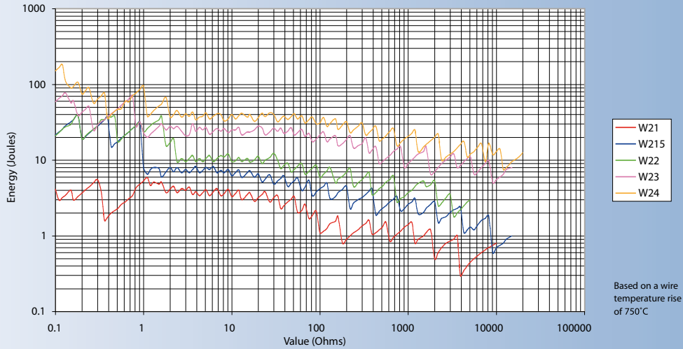
W20 Series "Overload Rating" Graph
