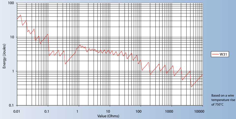
W31 Series "Energy Capability" Graph
