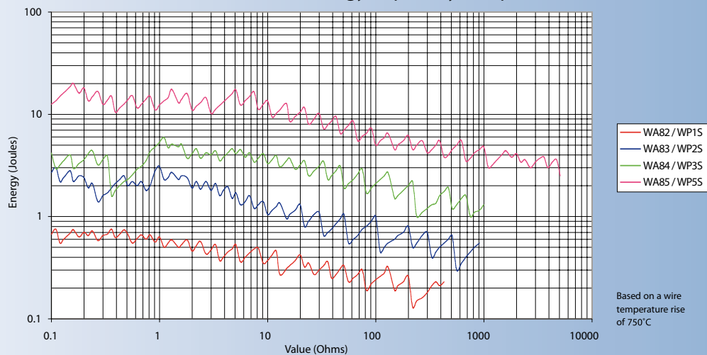
WA80 & WP-S Series "Energy Capability" Graph
