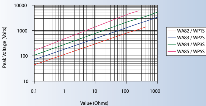
WA80 & WP-S Series 1.2/50 µs Graph
