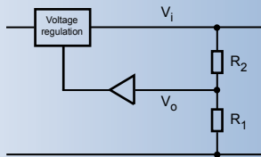
Figure 8 Voltage Divider
