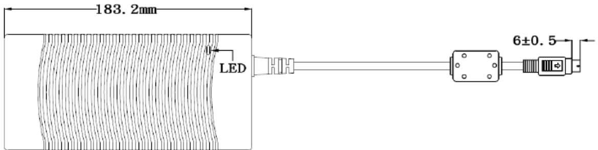
TOP-VIEW
